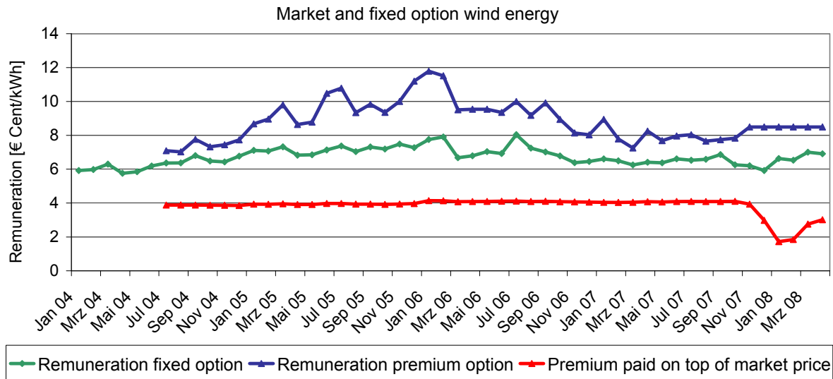
Figure 3.19: Remuneration for electricity from wind energy in Spain from January 2004 to March 2008
