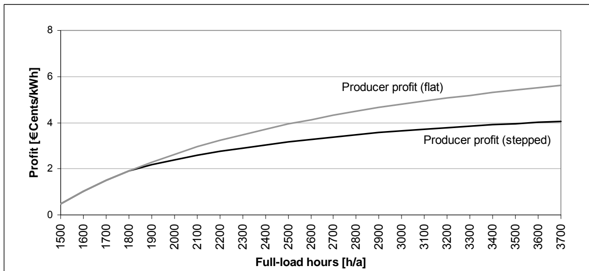
Figure 3.10: Producer profit for electricity from onshore wind energy in the Netherlands in 2006
