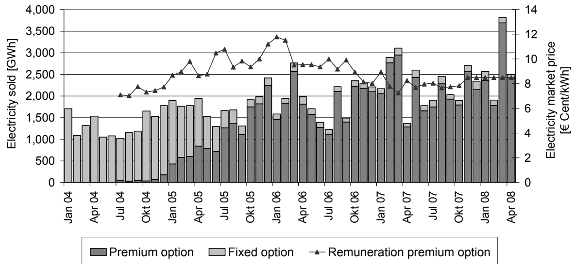
Figure 3.20: Electricity from wind energy sold within the fixed and the premium option.
