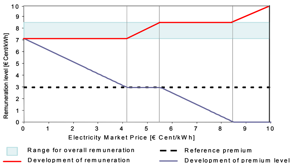
Figure 3.22: Progression of the remuneration level for wind onshore within the market option
