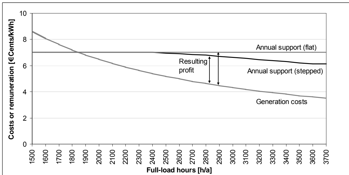
Figure 3.11: Electricity generation costs and annual support for onshore wind turbines in France in 2006 11
