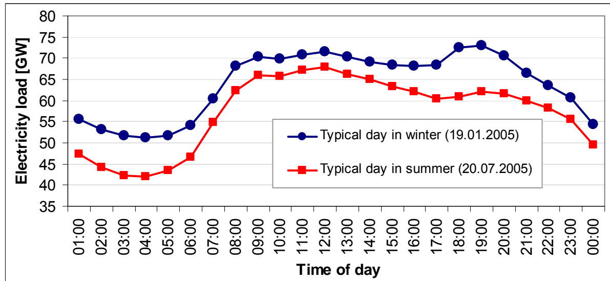
Figure 3.24: Typical electricity load curve
